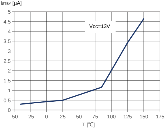
Standby current
